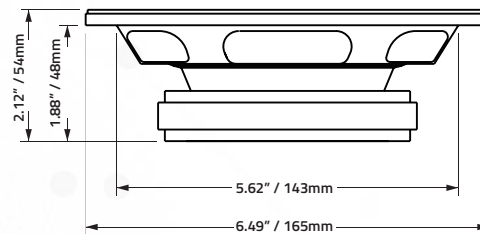
HM65PRO4 - MIDRANGE
