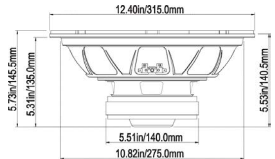
Recommended Air Space Sealed 1.15 cu. ft. / Vented 1.42 cu. ft.
